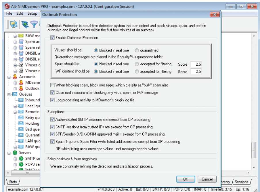
Configuration screen for Outbreak Protection.
